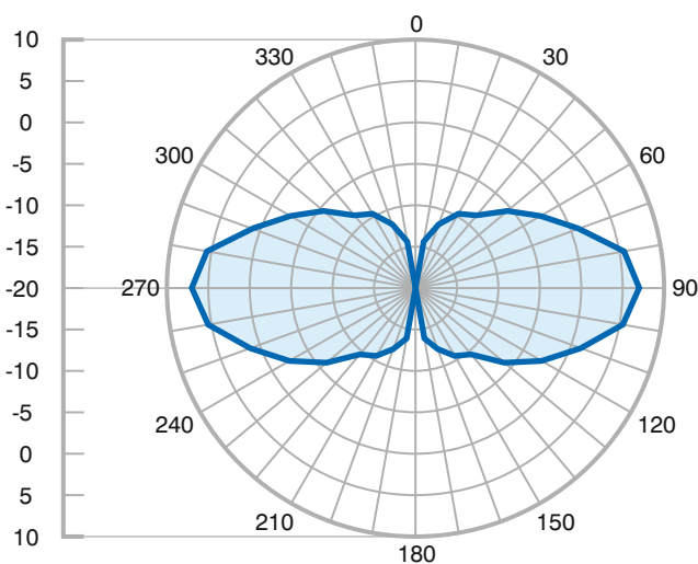
Vertical @ 1.3GHz
