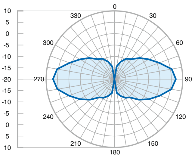
Vertical @ 1.5GHz
