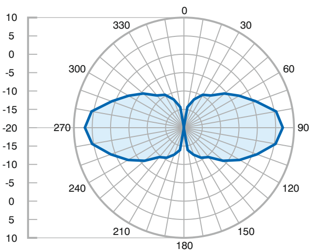
Vertical @ 1.5GHz
