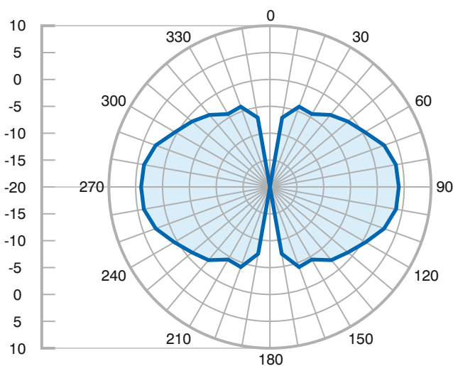
Vertical @ 1.4GHz
