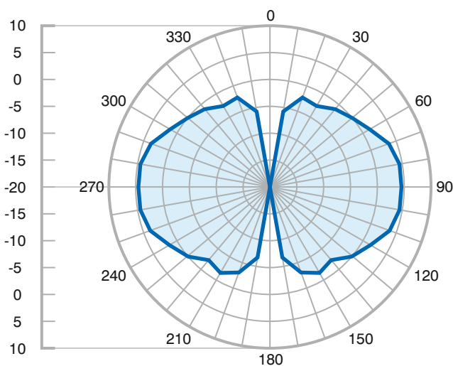
Vertical @ 2.4GHz
