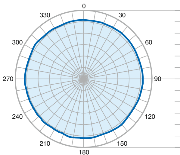
Horizontal @ 2.4GHz
