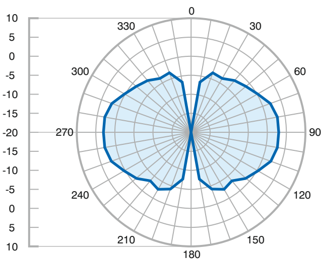
Vertical @ 1.4GHz
