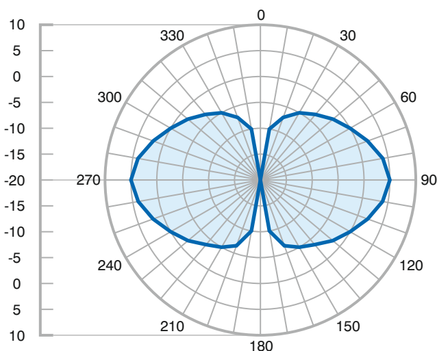
Vertical @ 5.8GHz
