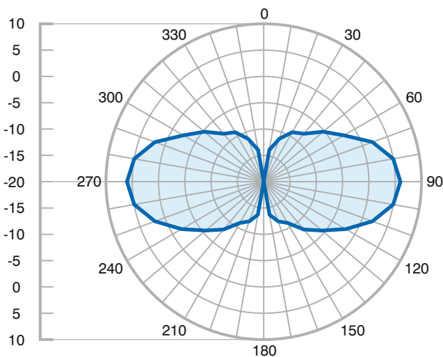
Vertical @ 2.4GHz
