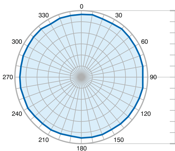
Horizontal @ 1.5GHz
