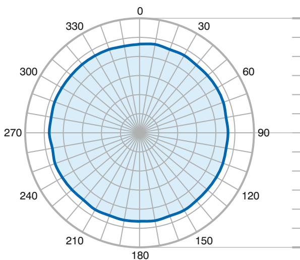
Horizontal @ 1.4GHz
