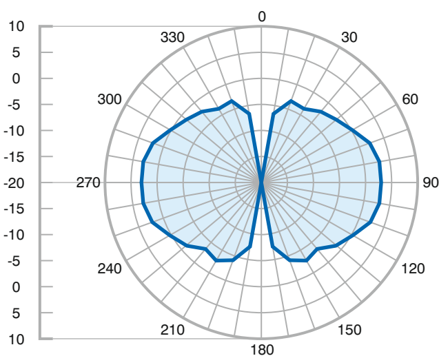
Vertical @ 5.8GHz
