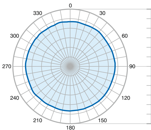
Horizontal @ 2.4GHz
