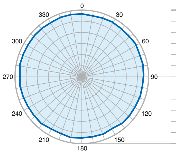
Horizontal @ 1.3GHz
