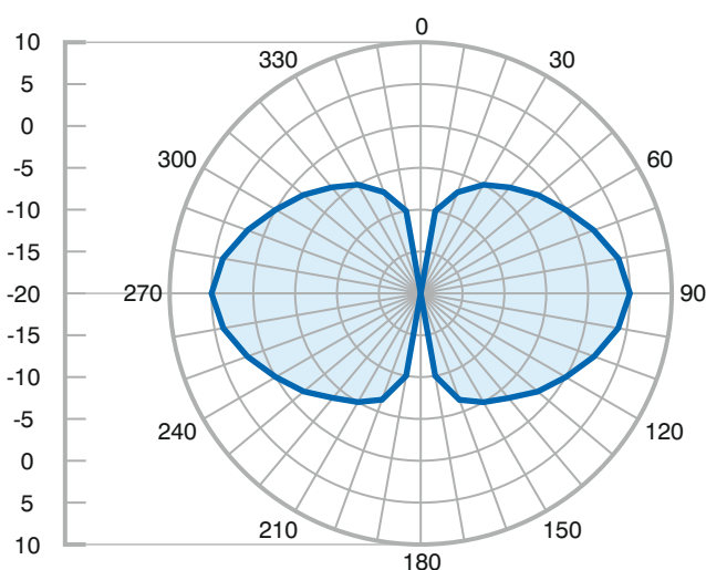
Vertical @ 5.8GHz
