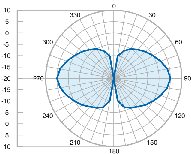
Vertical @ 5.8GHz
