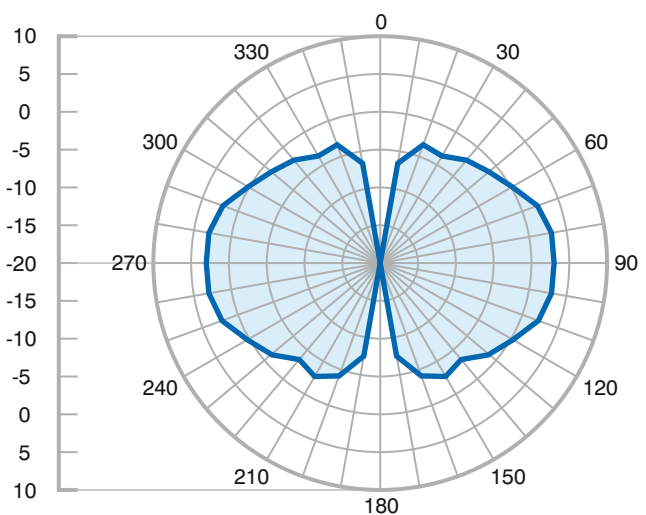
Vertical @ 1.4GHz
