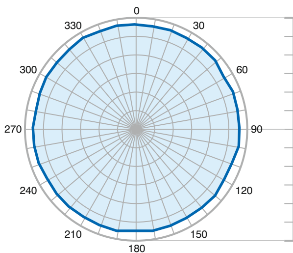
Horizontal @ 1.3GHz
