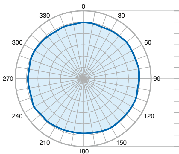
Horizontal @ 1.4GHz
