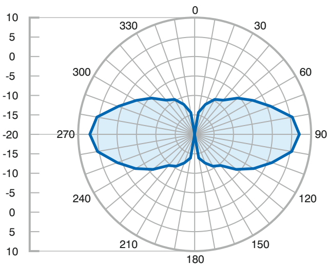
Vertical @ 1.3GHz
